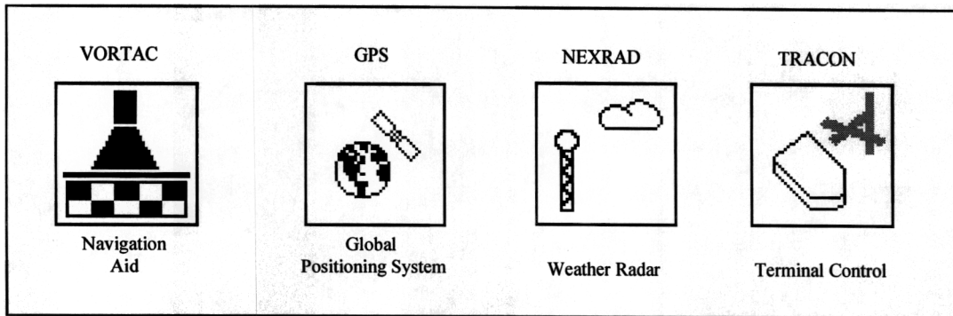
Figure 14. Typical icons.
