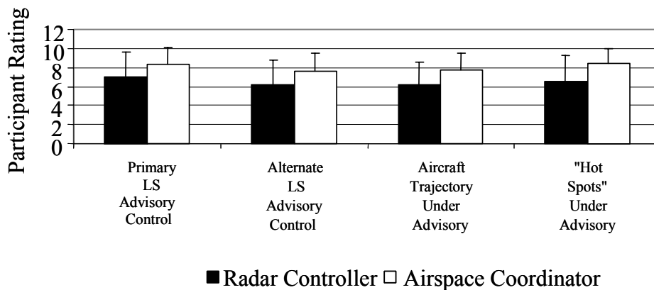
Figure 34. Importance of primary LS advisory control action and alternate LS advisory control action for each aircraft, aircraft trajectory under advisory route, and “hot spots” under advisory route by ATCS role.
